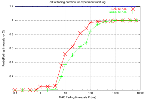
Fig. 3. cdf of MAC fading timescale: slow fading.
