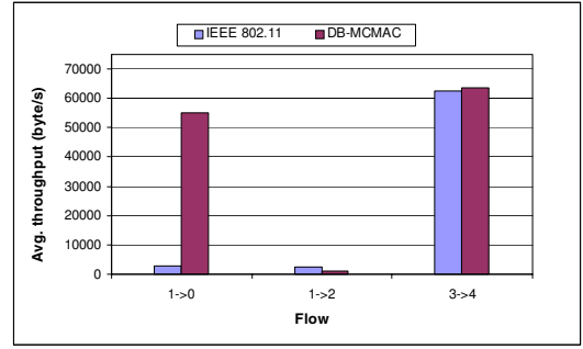
Fig. 16. Multi-receiver diversity gain: interference.
