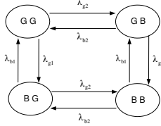
Fig. 9. Markov chain model for two independent fading channels.
