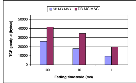
Fig. 24. TCP performance against fading timescale.
