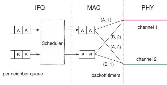
Fig. 7. Architecture of the DB-MCMAC protocol.
