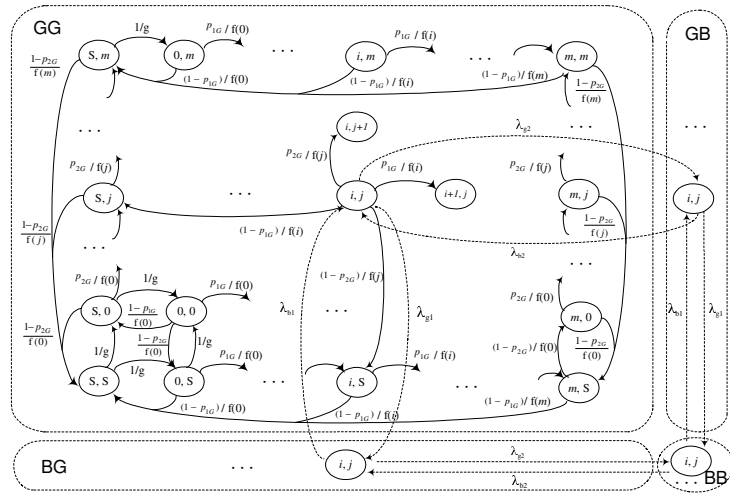
Fig. 10. Markov chain model of DB-MCMAC for the scenario shown in Fig.8.
