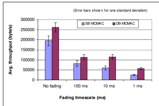
Fig. 25. MAC diversity gains with random scenarios: 11 Mbps data rate
