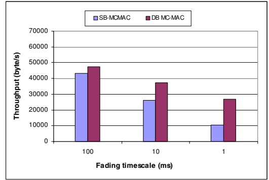
Fig. 18. Multi-channel diversity gains in fast fading (three channels).
