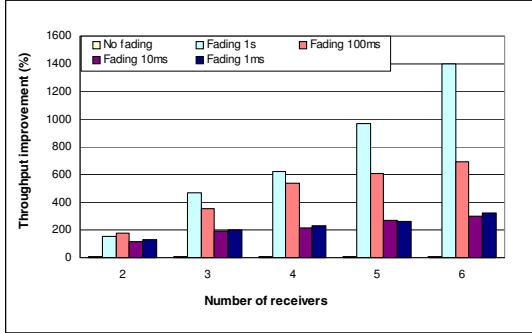
Fig. 14. Multi-receiver diversity gain against number of receivers.
