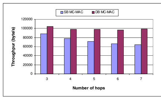
Fig. 23. Intra-flow interference mitigation against the number of hops.
