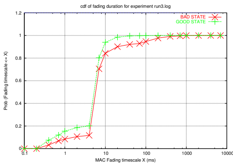
Fig. 2. cdf of MAC fading timescale: fast fading.
