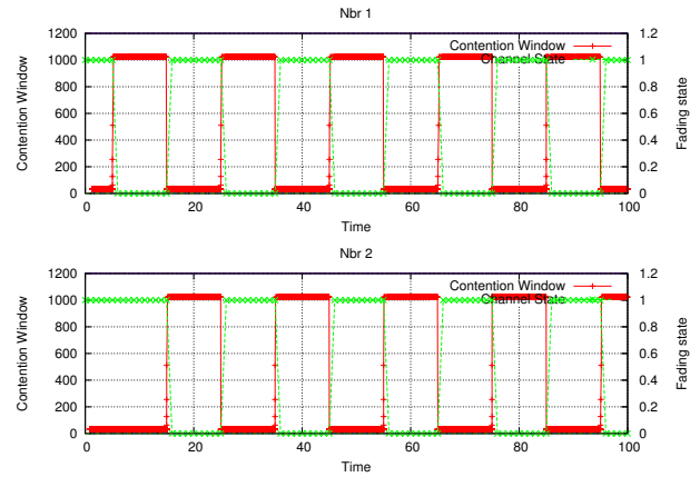
Fig. 12. Tracking the fading condition: CW adaptation with NAV overriding.
