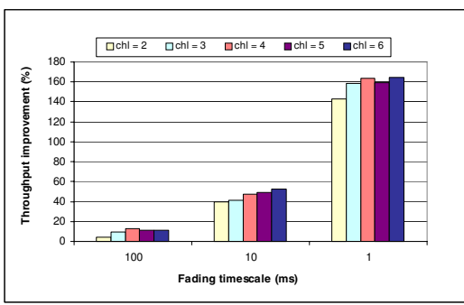
Fig. 19. Multi-channel diversity gains against fading timescale as the number of channels increases.
