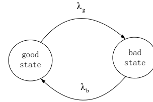
Fig. 1. Two state Markov fading model.
